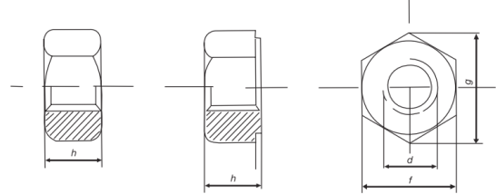
DIMENSION (mm) AND WEIGHT (Kg) PER 100 PIECES (IMPERIAL SIZE)
